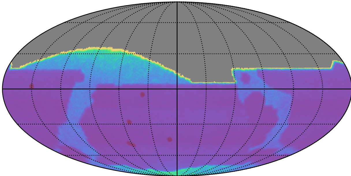
weather_cloudso12v3.4_10yrs : Proper Motion Uncert @ 20.5
