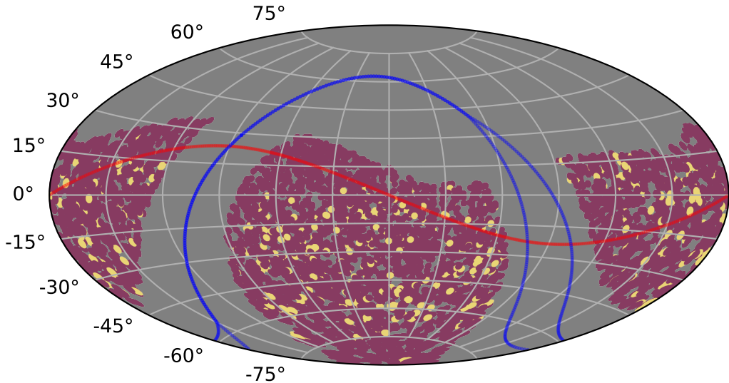
weather_cloudso12v3.4_10yrs : PrestoKNe_presto_color_detect
