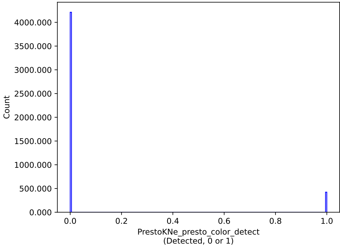
weather_cloudso12v3.4_10yrs : PrestoKNe_presto_color_detect
