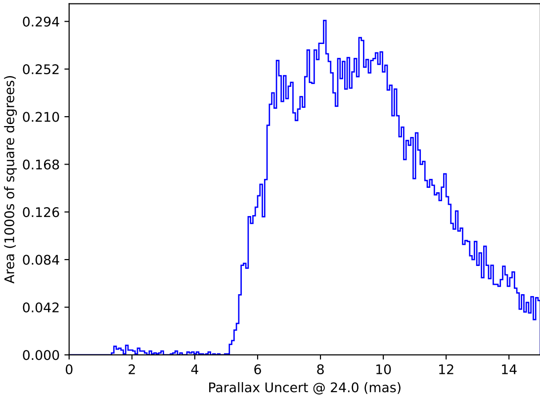
weather_cloudso12v3.4_10yrs : Parallax Uncert @ 24.0
