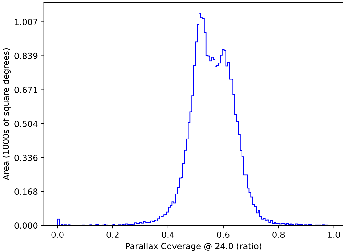
weather_cloudso12v3.4_10yrs : Parallax Coverage @ 24.0
