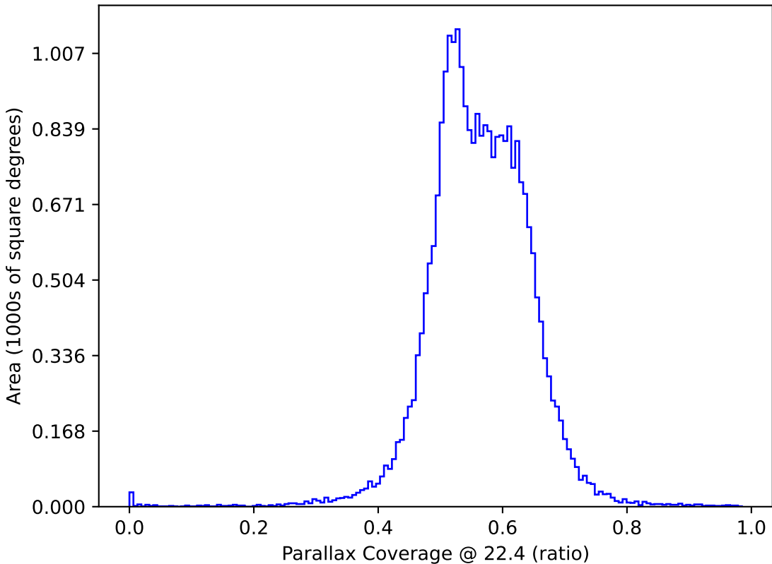
weather_cloudso12v3.4_10yrs : Parallax Coverage @ 22.4
