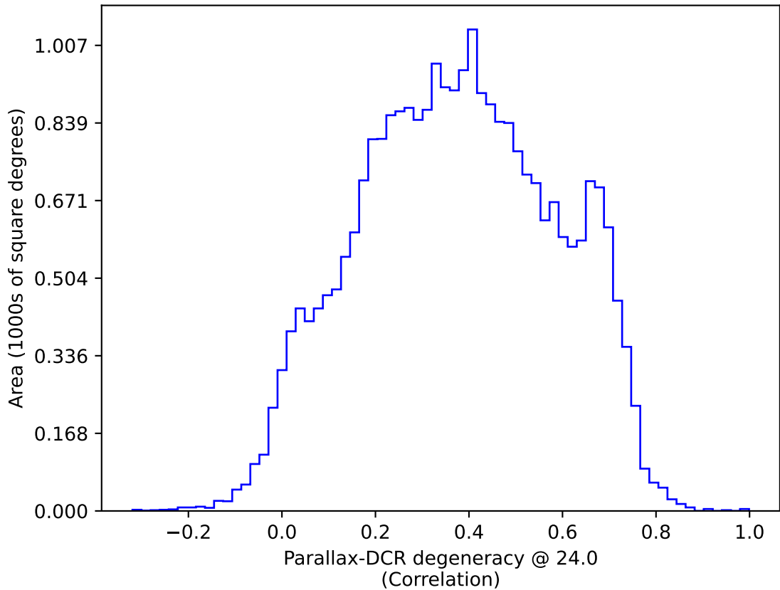
weather_cloudso12v3.4_10yrs : Parallax-DCR degeneracy @ 24.0
