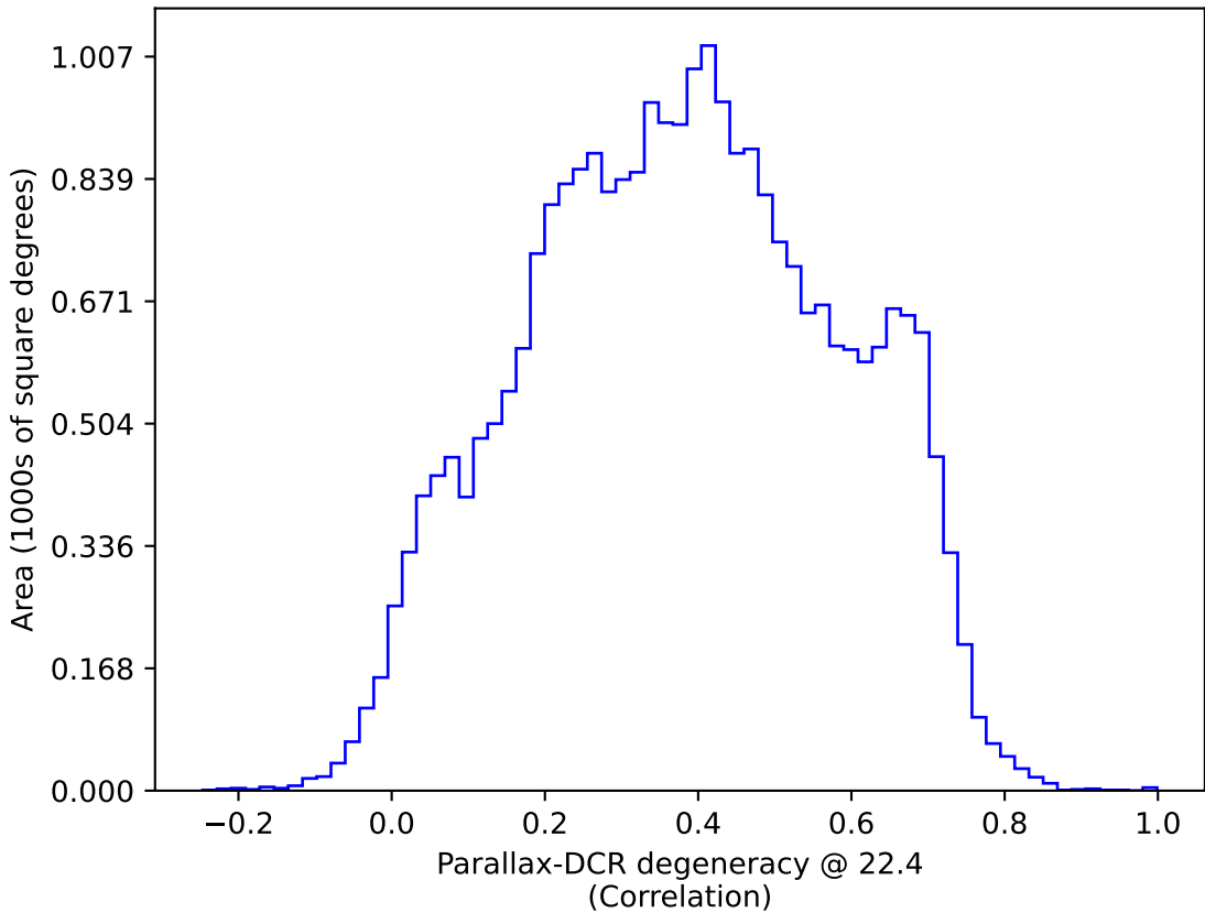
weather_cloudso12v3.4_10yrs : Parallax-DCR degeneracy @ 22.4
