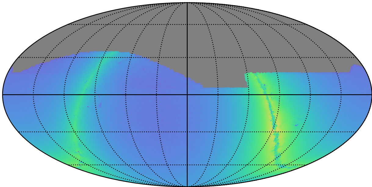
weather_cloudso12v3.4_10yrs z: Nstars_no_crowding
