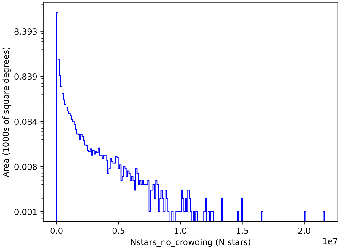
weather_cloudso12v3.4_10yrs r: Nstars_no_crowding
