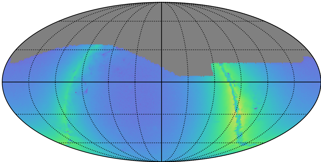
weather_cloudso12v3.4_10yrs g: Nstars_no_crowding
