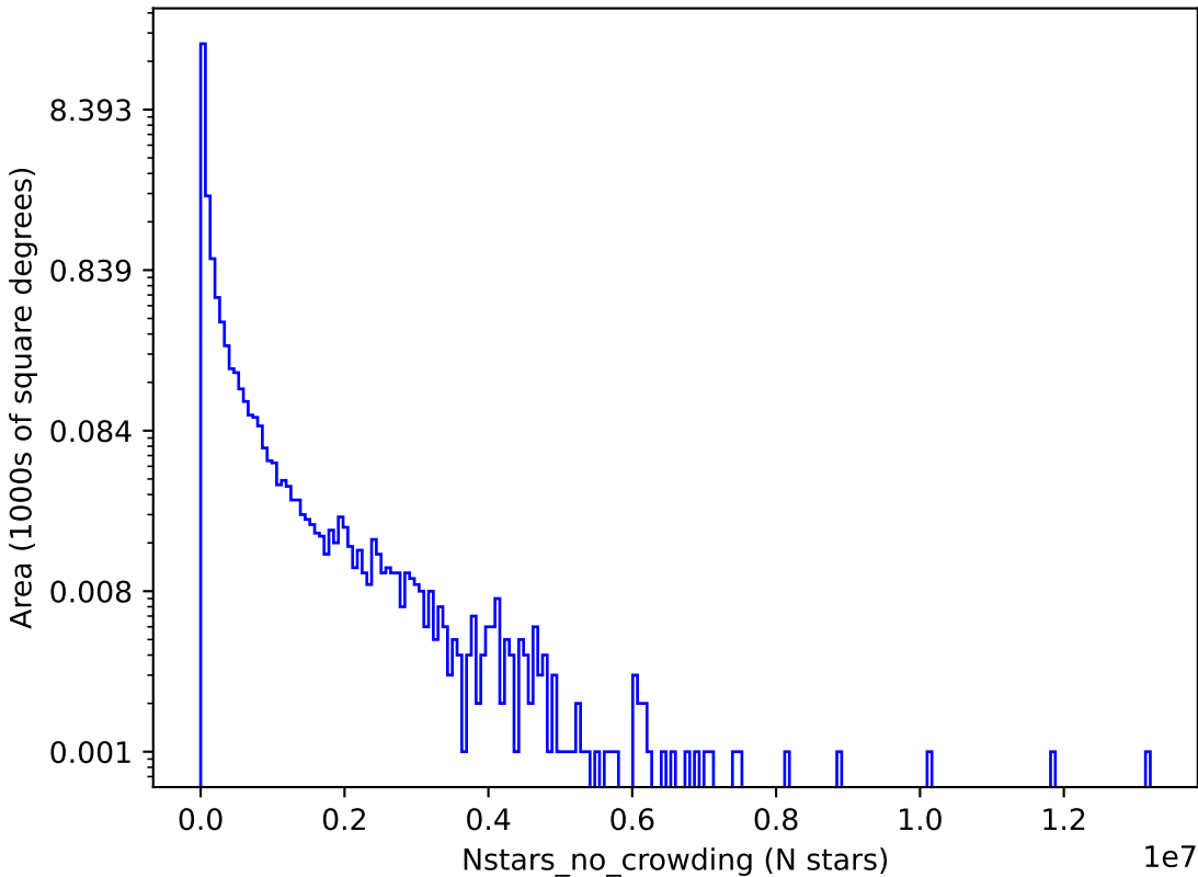
weather_cloudso12v3.4_10yrs g: Nstars_no_crowding
