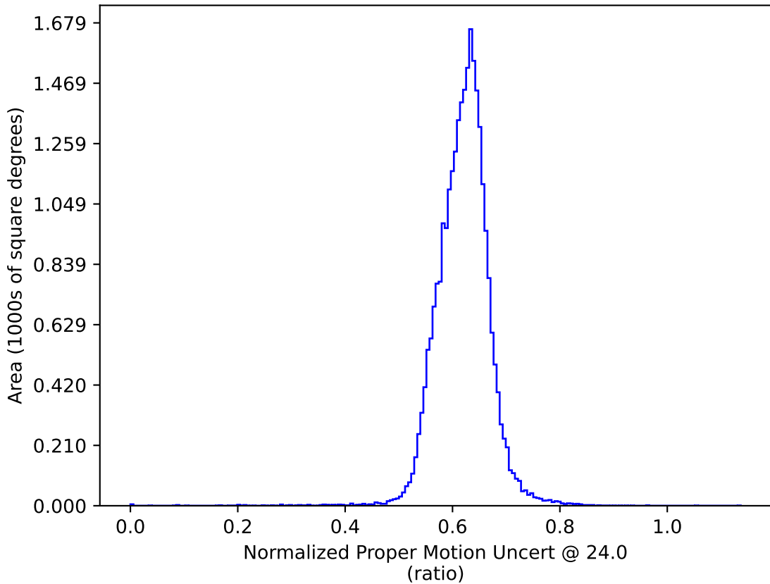
weather_cloudso12v3.4_10yrs : Normalized Proper Motion Uncert @ 24.0
