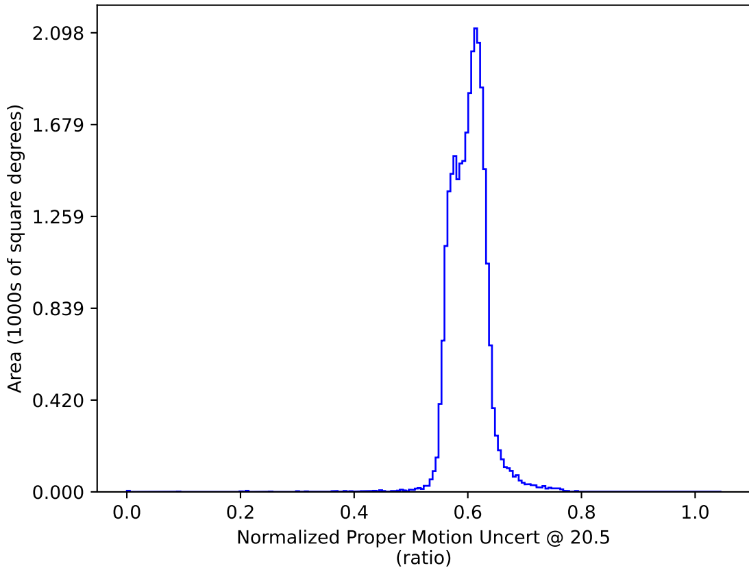
weather_cloudso12v3.4_10yrs : Normalized Proper Motion Uncert @ 20.5
