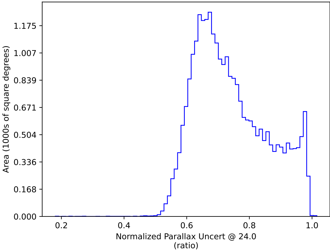
weather_cloudso12v3.4_10yrs : Normalized Parallax Uncert @ 24.0
