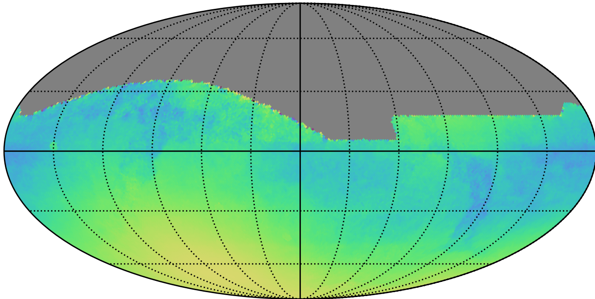
weather_cloudso12v3.4_10yrs : Normalized Parallax Uncert @ 22.4
