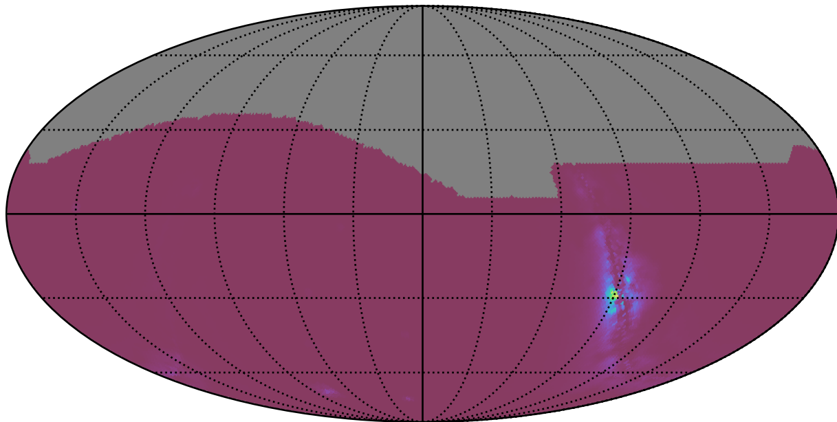
weather_cloudso12v3.4_10yrs : NlcPoints
