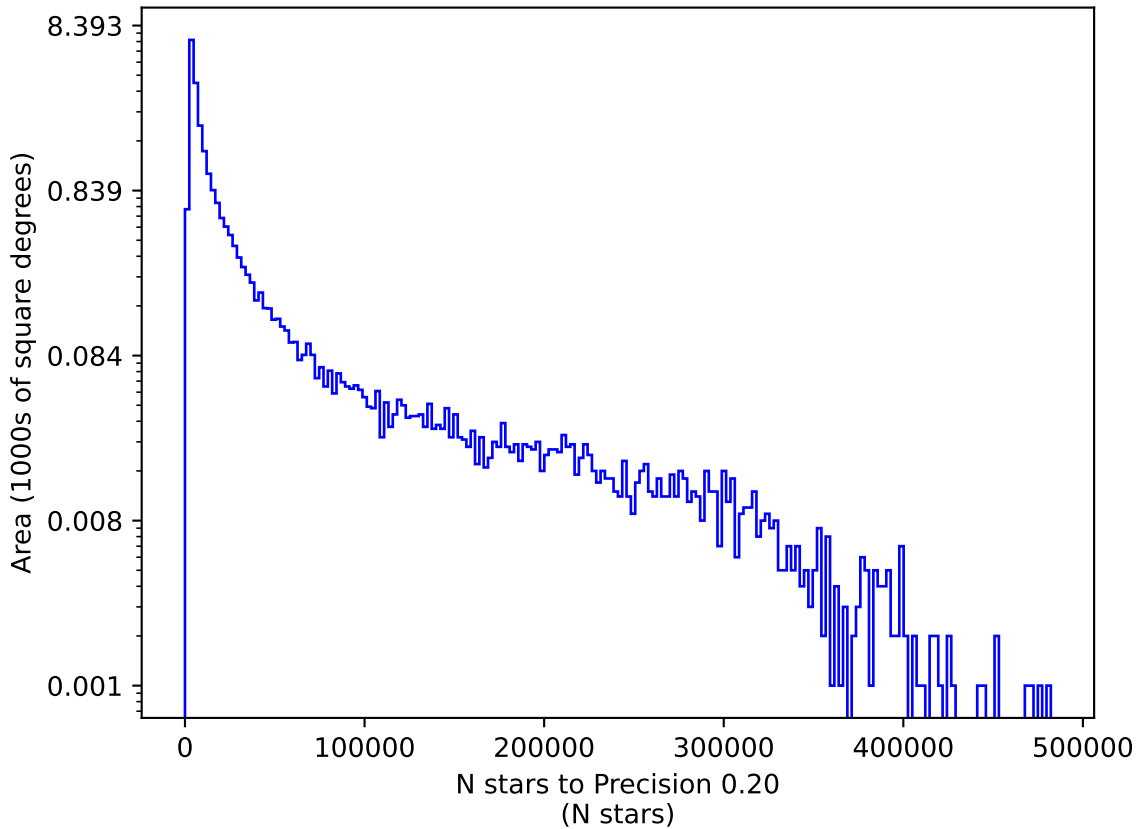
weather_cloudso12v3.4_10yrs u: N stars to Precision 0.20
