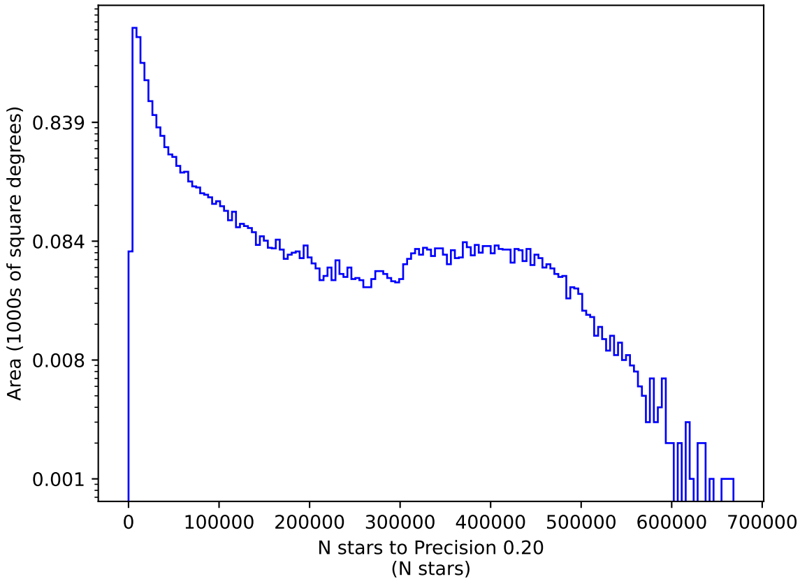
weather_cloudso12v3.4_10yrs r: N stars to Precision 0.20
