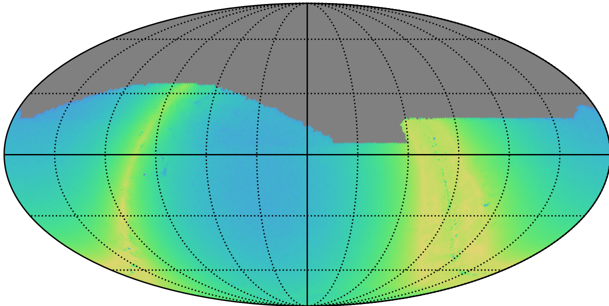
weather_cloudso12v3.4_10yrs i: N stars to Precision 0.20
