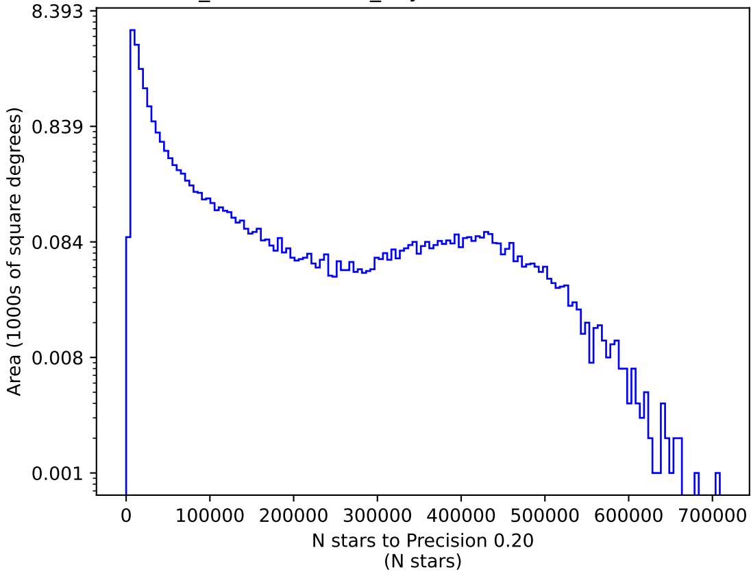
weather_cloudso12v3.4_10yrs i: N stars to Precision 0.20
