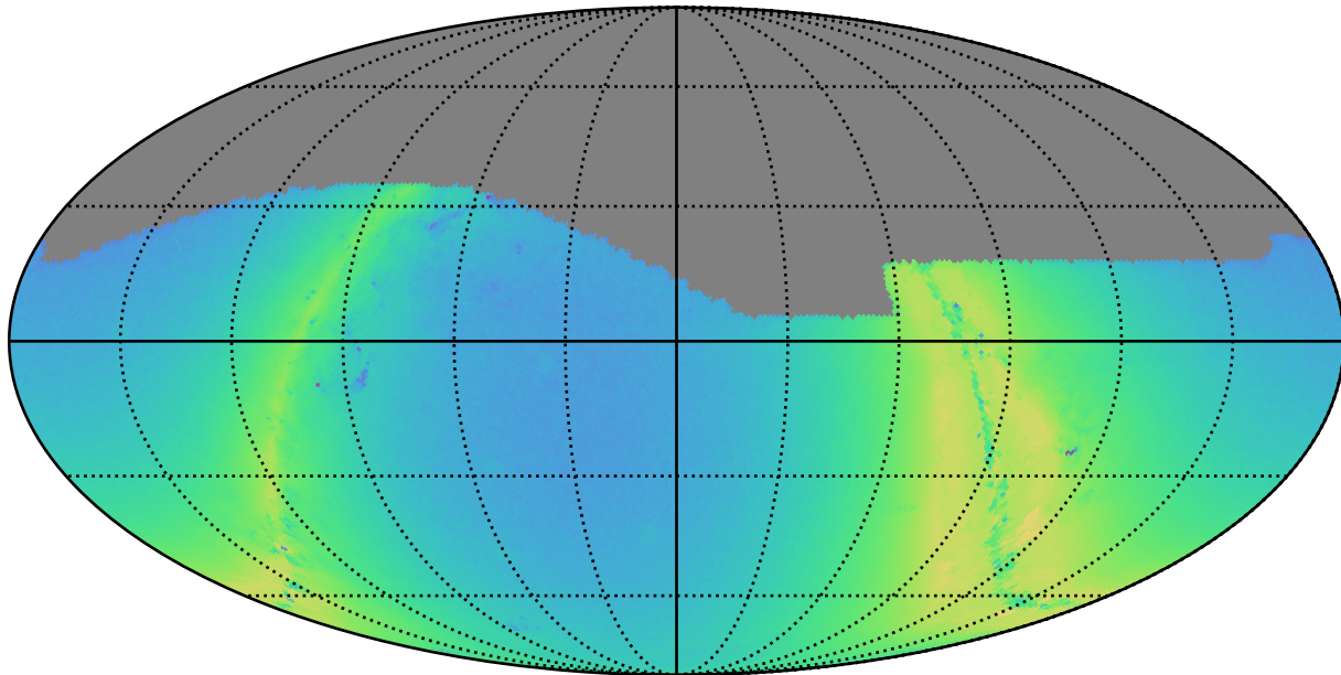
weather_cloudso12v3.4_10yrs g: N stars to Precision 0.20
