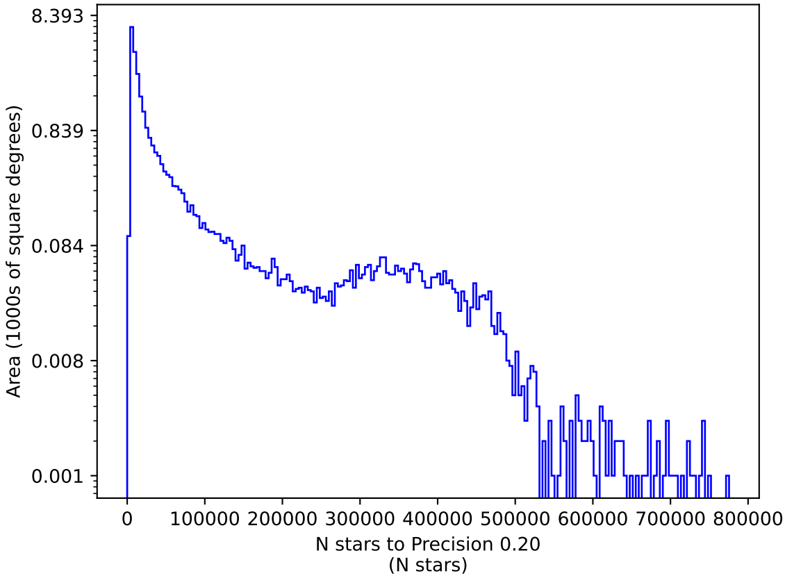
weather_cloudso12v3.4_10yrs g: N stars to Precision 0.20
