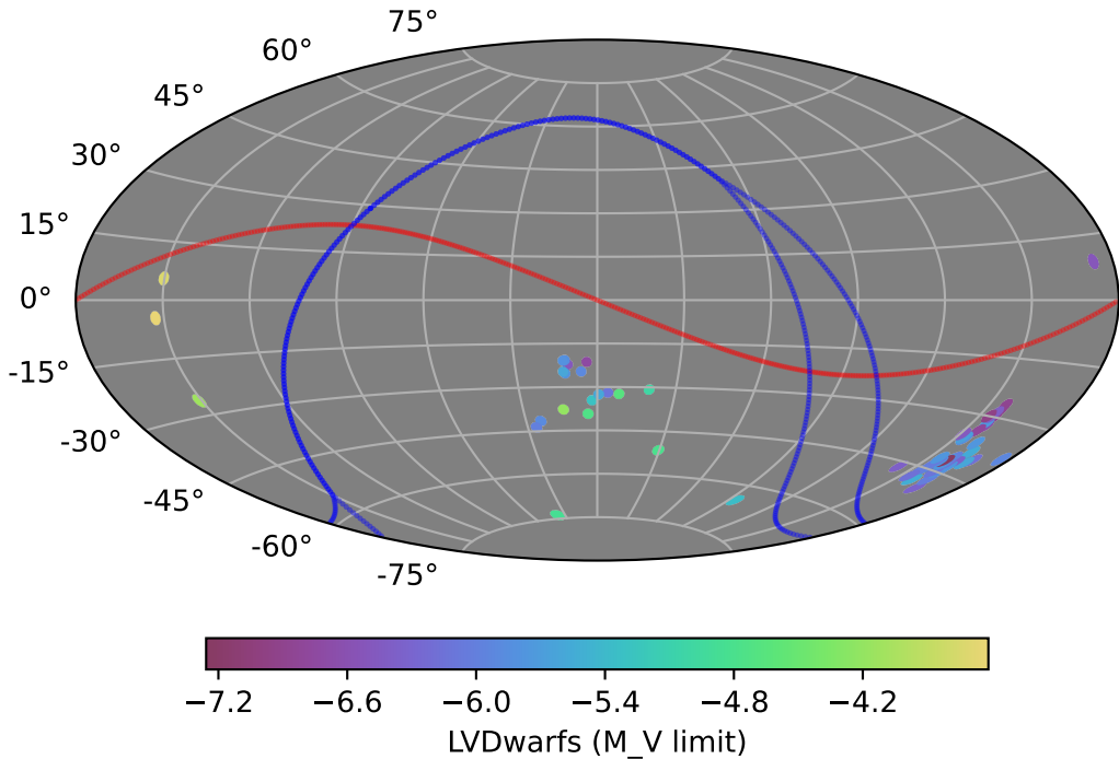
weather_cloudso12v3.4_10yrs gi: LVDwarfs
