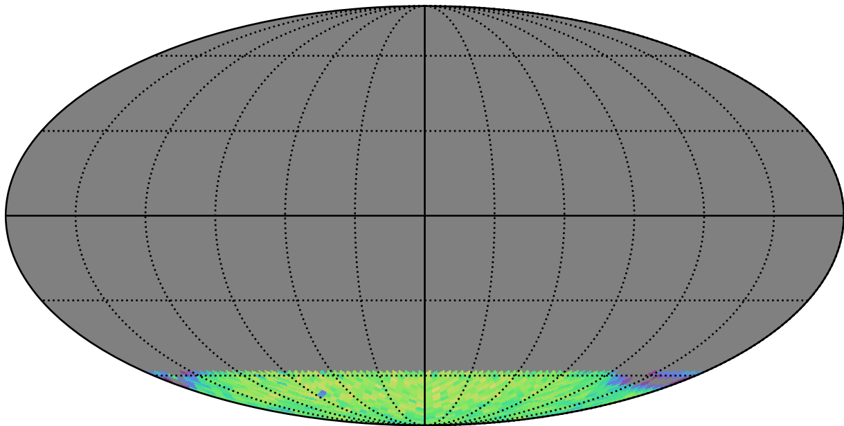
weather_cloudso12v3.4_10yrs gi SCP: LVDwarfs
