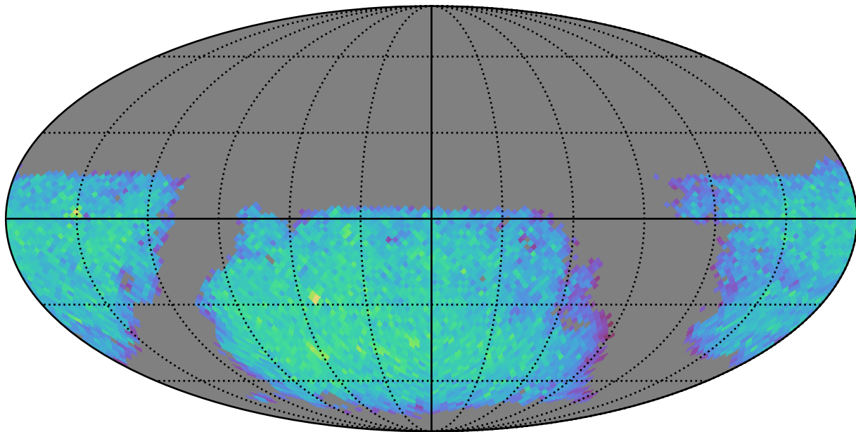
weather_cloudso12v3.4_10yrs gi: LVDwarfs
