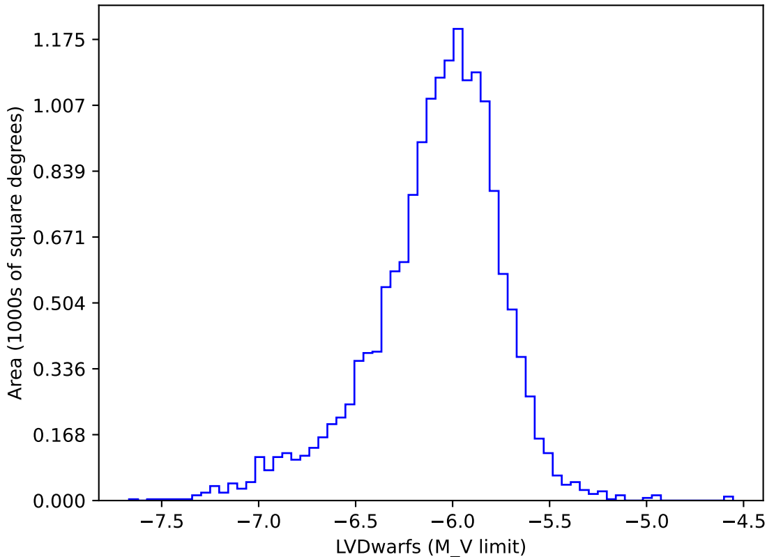
weather_cloudso12v3.4_10yrs gi: LVDwarfs
