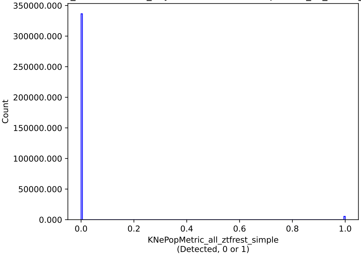
weather_cloudso12v3.4_10yrs all models: KNePopMetric_all_ztfrest_simple
