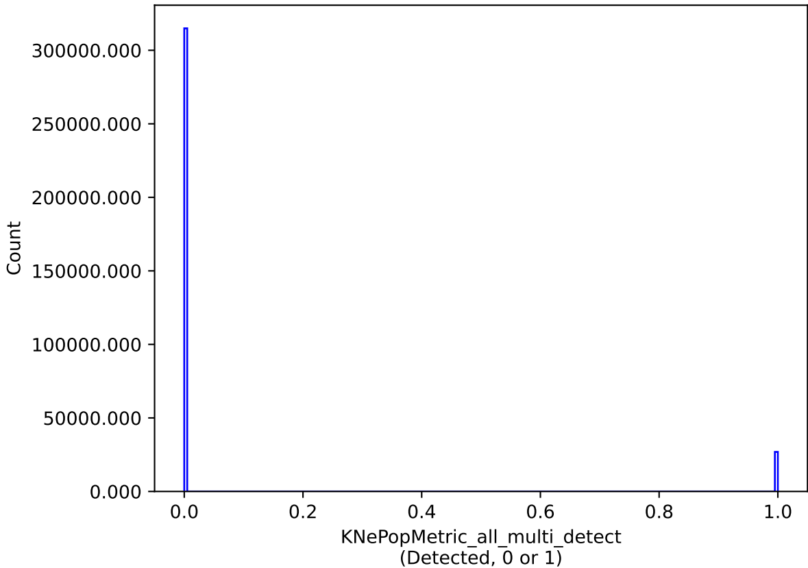
weather_cloudso12v3.4_10yrs all models: KNePopMetric_all_multi_detect
