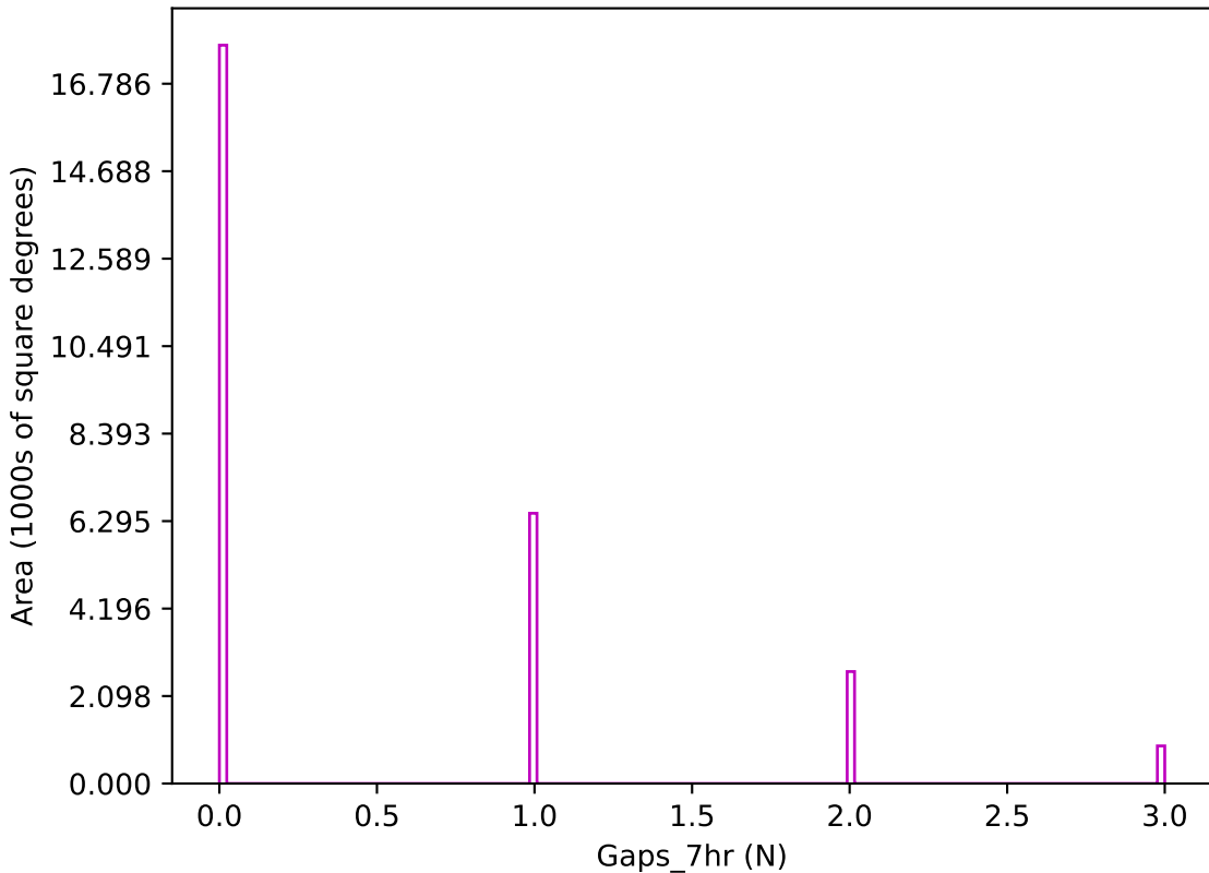
weather_cloudso12v3.4_10yrs z band: Gaps_7hr
