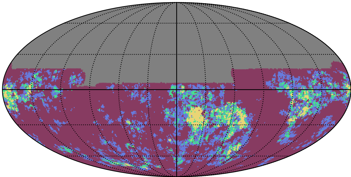
weather_cloudso12v3.4_10yrs y band: Gaps_7hr
