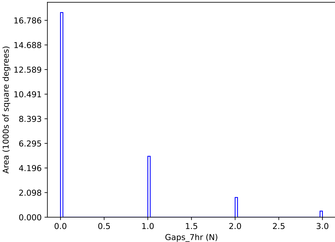
weather_cloudso12v3.4_10yrs y band: Gaps_7hr
