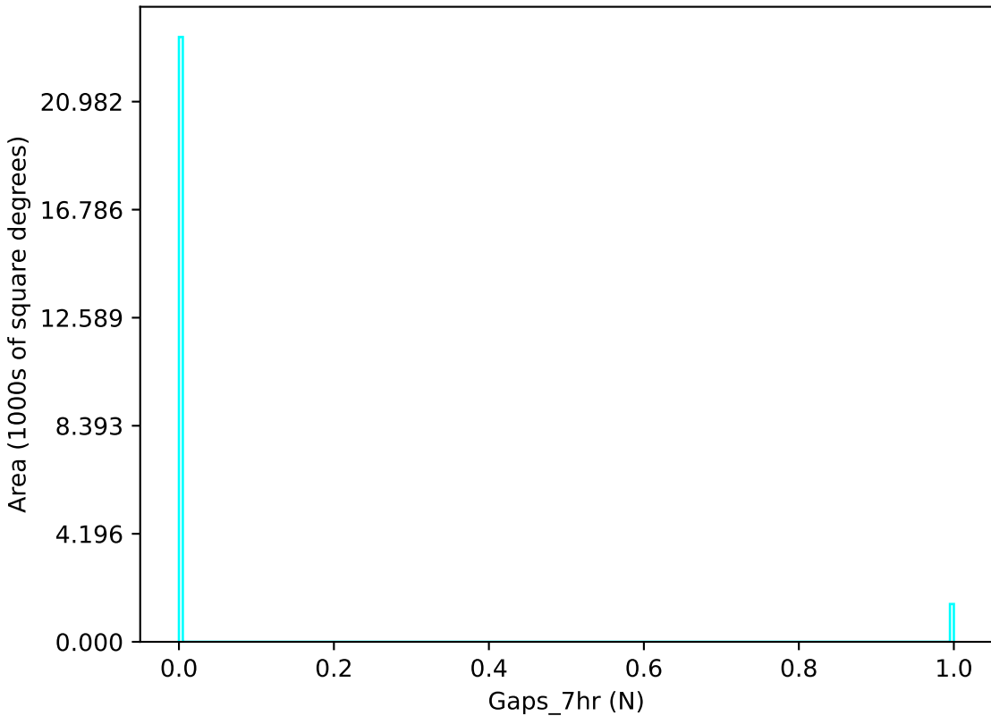
weather_cloudso12v3.4_10yrs u band: Gaps_7hr
