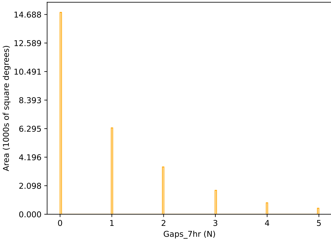
weather_cloudso12v3.4_10yrs r band: Gaps_7hr
