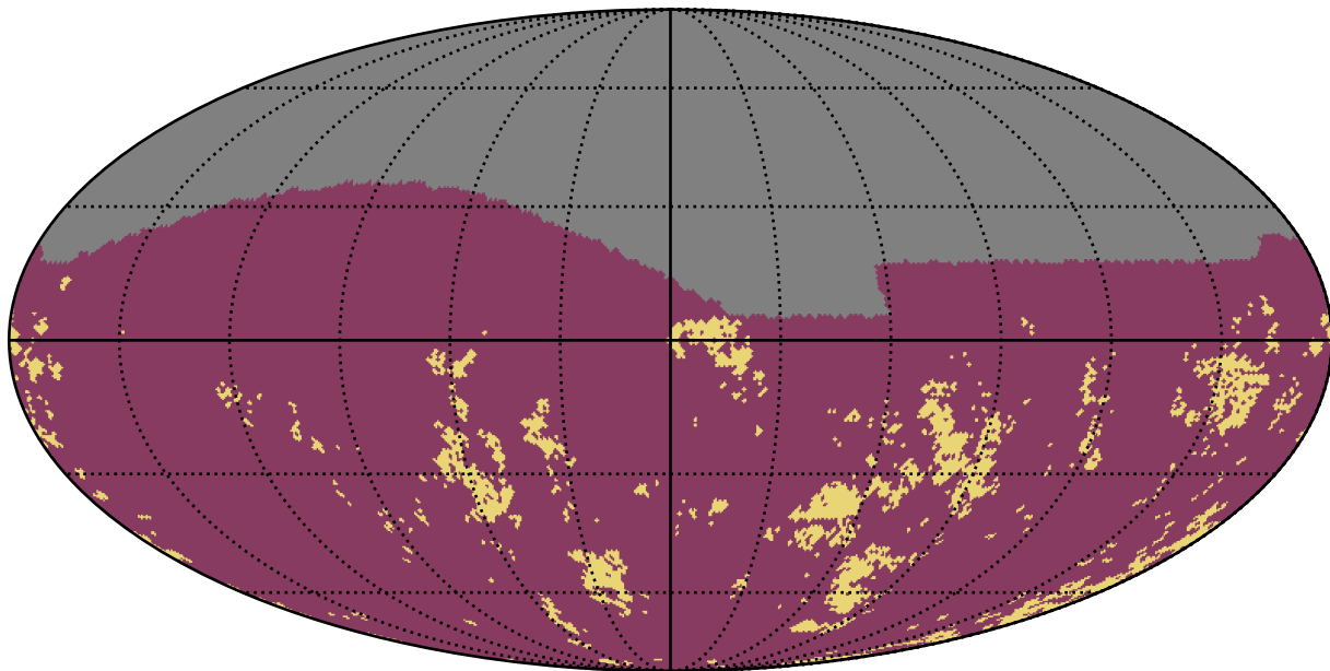
weather_cloudso12v3.4_10yrs g band: Gaps_7hr
