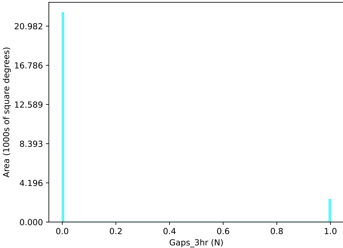
weather_cloudso12v3.4_10yrs u band: Gaps_3hr
