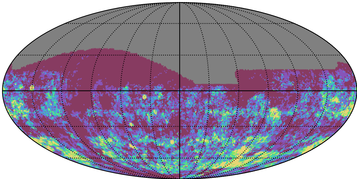
weather_cloudso12v3.4_10yrs r band: Gaps_3hr
