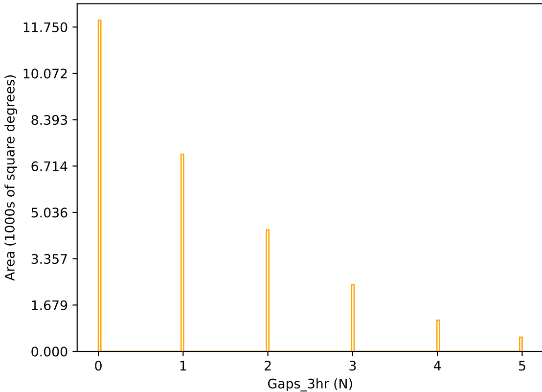
weather_cloudso12v3.4_10yrs r band: Gaps_3hr
