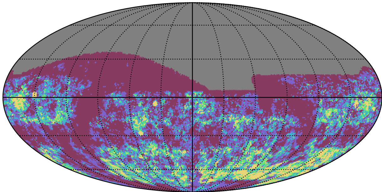
weather_cloudso12v3.4_10yrs i band: Gaps_3hr
