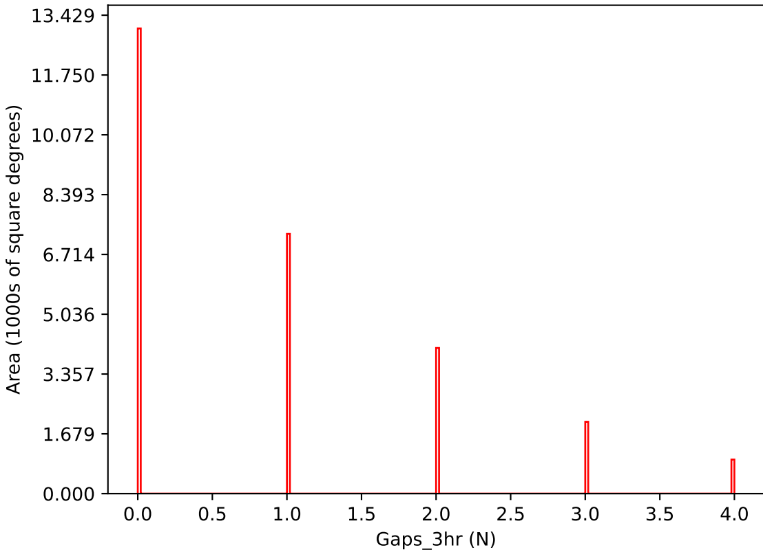
weather_cloudso12v3.4_10yrs i band: Gaps_3hr
