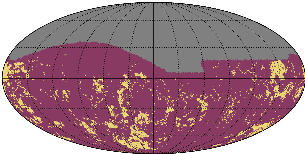
weather_cloudso12v3.4_10yrs g band: Gaps_3hr
