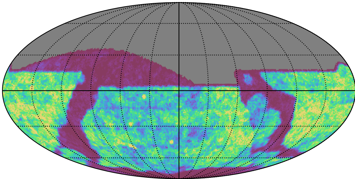
weather_cloudso12v3.4_10yrs z band: Gaps_24hr
