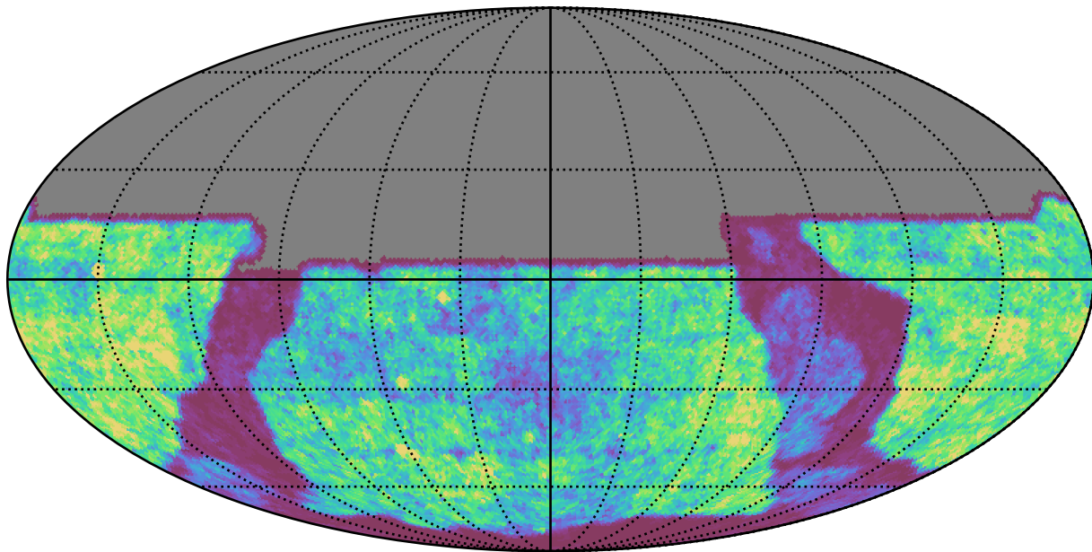
weather_cloudso12v3.4_10yrs y band: Gaps_24hr
