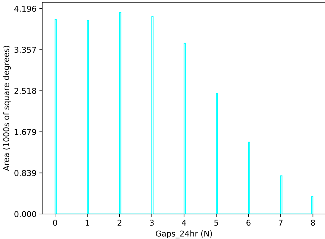
weather_cloudso12v3.4_10yrs u band: Gaps_24hr
