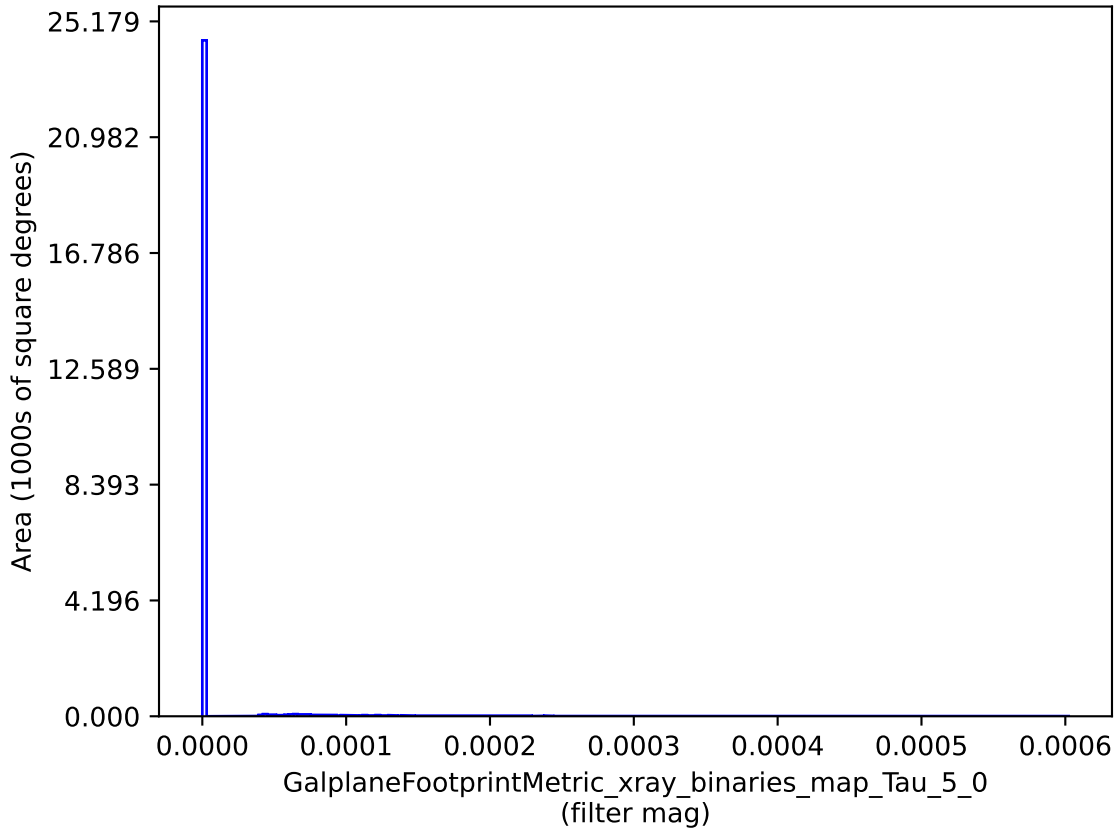
weather_cloudso12v3.4_10yrs : GalplaneFootprintMetric_xray_binaries_map_Tau_5_0
