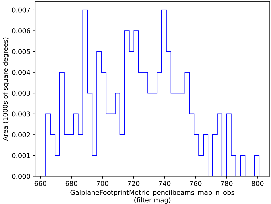
weather_cloudso12v3.4_10yrs : GalplaneFootprintMetric_pencilbeams_map_n_obs
