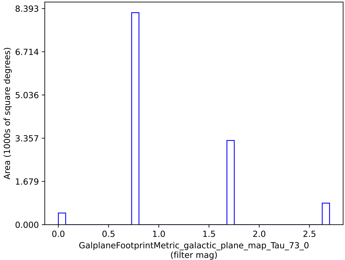
weather_cloudso12v3.4_10yrs : GalplaneFootprintMetric_galactic_plane_map_Tau_73_0
