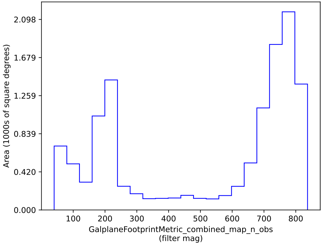
weather_cloudso12v3.4_10yrs : GalplaneFootprintMetric_combined_map_n_obs
