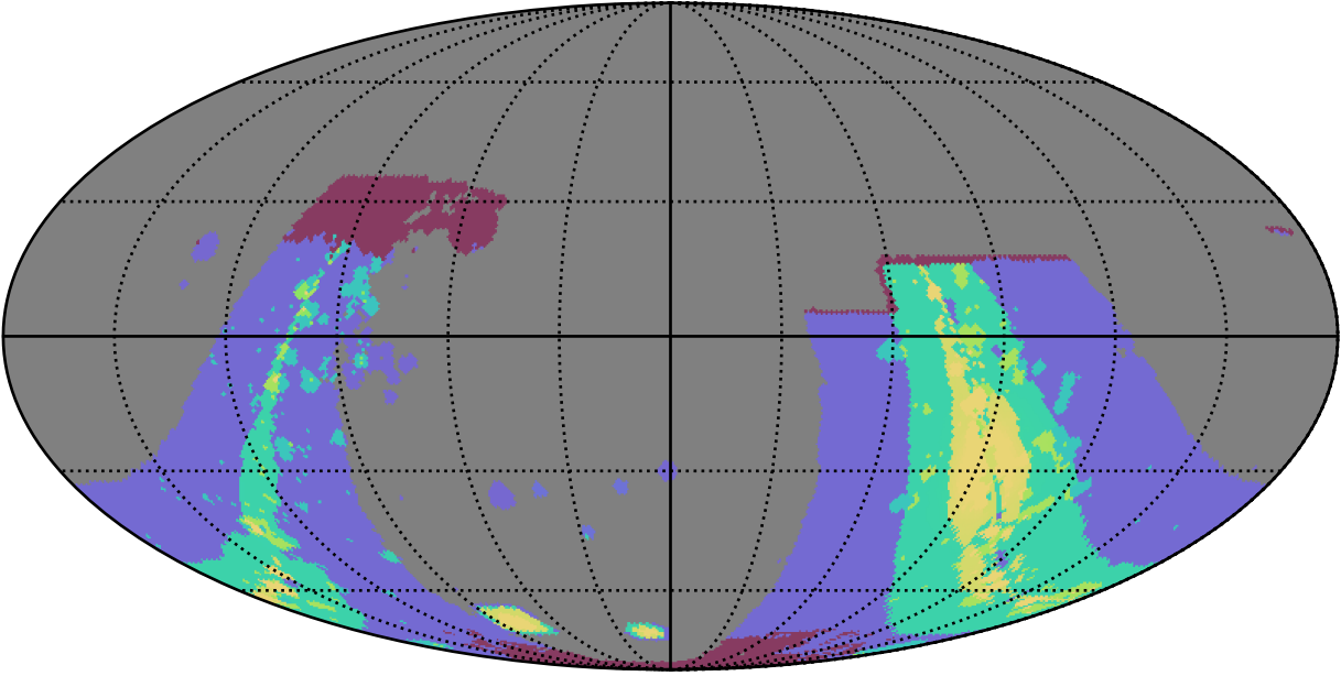
weather_cloudso12v3.4_10yrs : GalplaneFootprintMetric_combined_map_Tau_46_5
