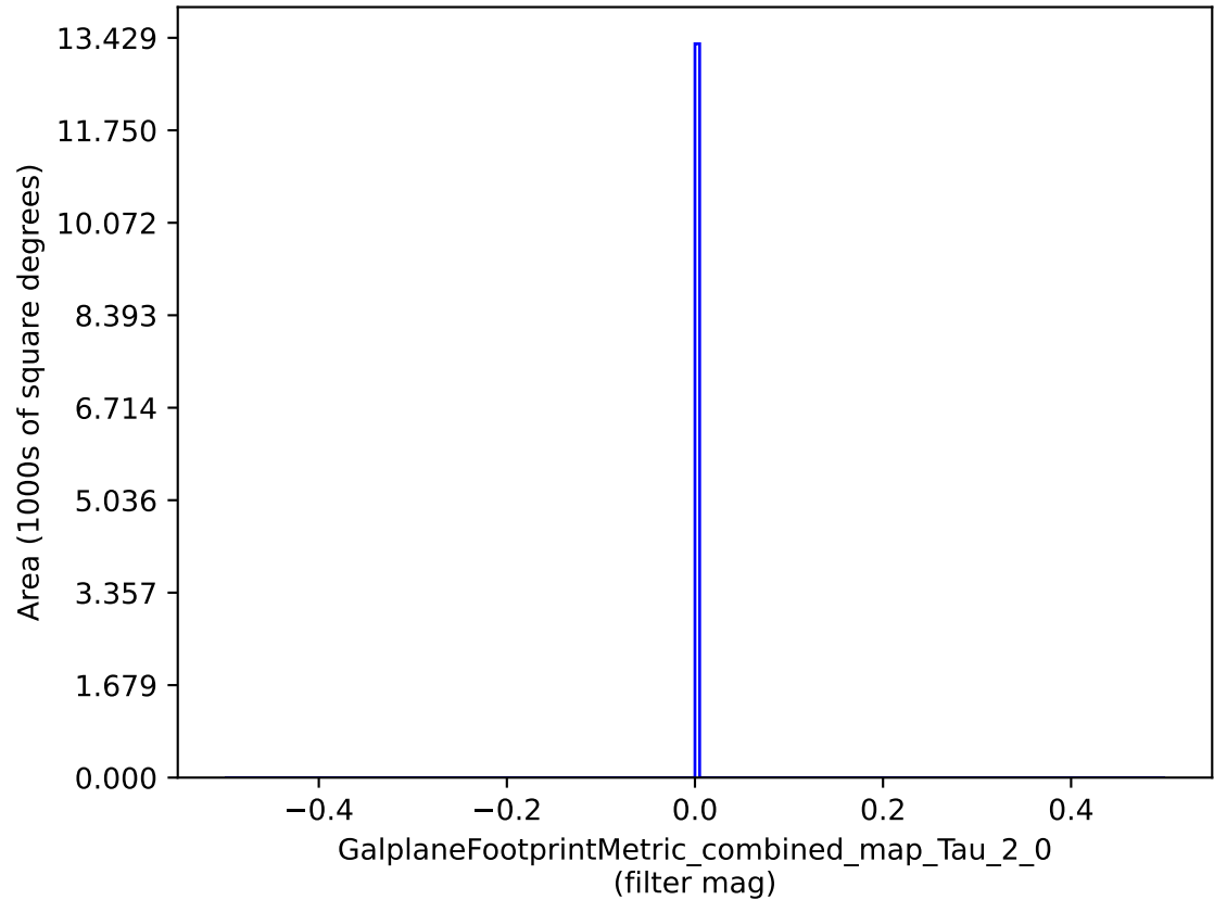
weather_cloudso12v3.4_10yrs : GalplaneFootprintMetric_combined_map_Tau_2_0
